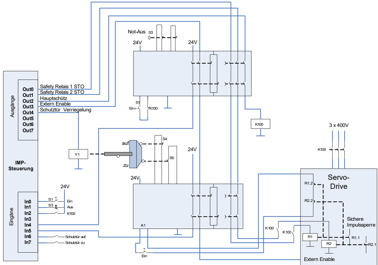
Fig.. 33: STO, locked safety door
