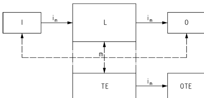
Fig. 25: Architecture, category 2
