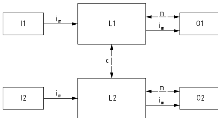
Fig. 26: Architecture, category 3
