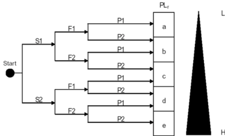
Fig. 18: Risk graph
