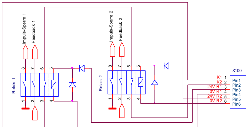
Fig. 8: Safety stop
