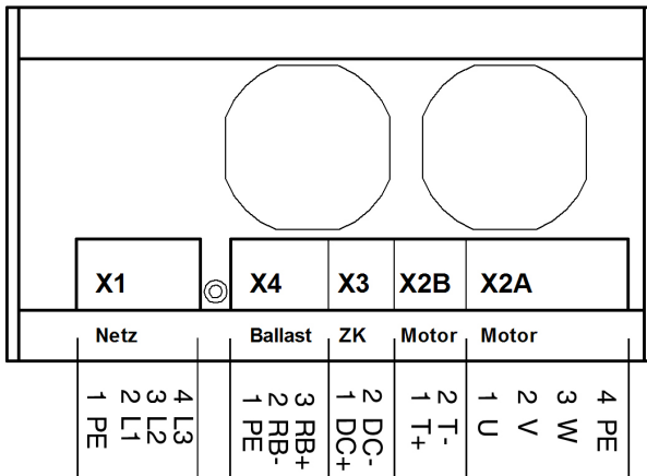
Fig. 11: Pin assignment 2
