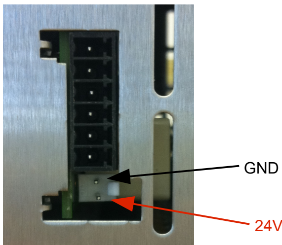
Fig. 6: Fan connection, SAC3x3
