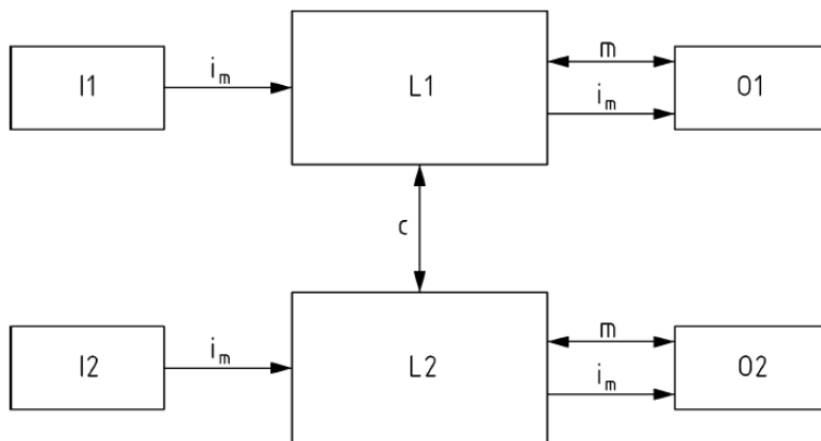
Fig. 27: Architecture, category 4
