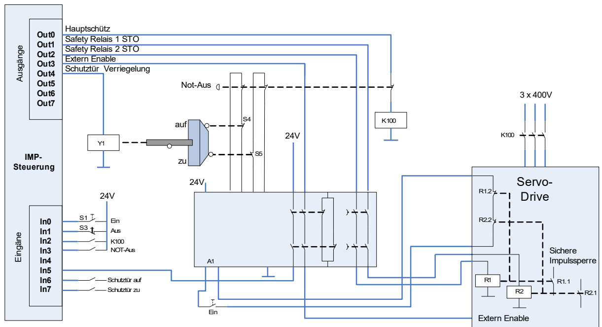
Fig. 34: STO with a safety switching device
