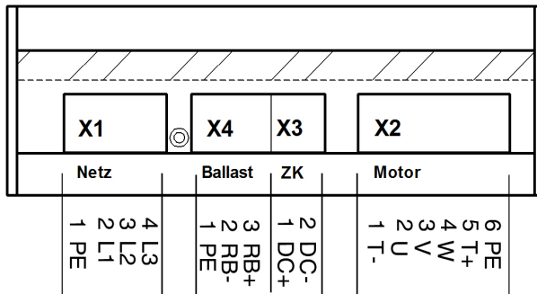
Fig. 10: Pin assignment 1
