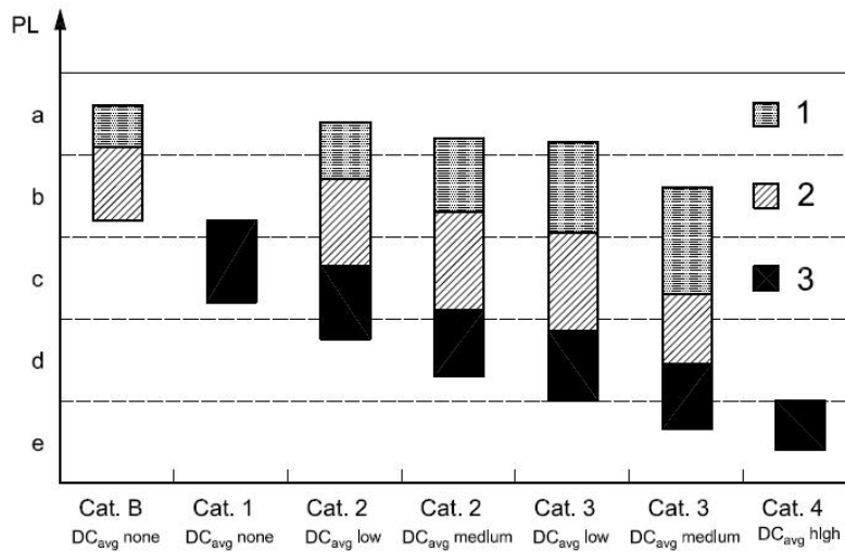
Fig. 28: Relationship between the categories DC, MTTFd of each channel and PL
