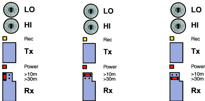
Fig. 15: No jumper, 10m jumper, 30m jumper
