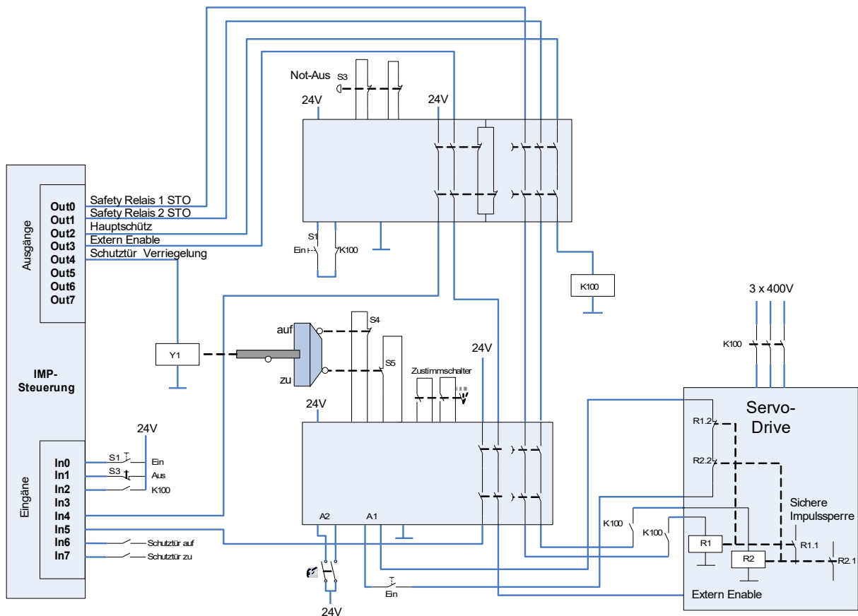
Fig. 35: STO with enabling button
