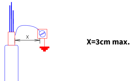
Fig. 6 Shield grounding using wire
