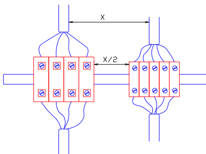
Fig. 11 Terminals
